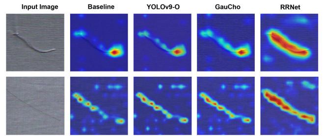
Fig. 5. Grad-CAM visualizations of representative elongated defects. Compared with the baseline, YOLOv9-O, and GauCho, RRNet produces more continuous defect-focused activations while suppressing responses to surrounding textile textures.
