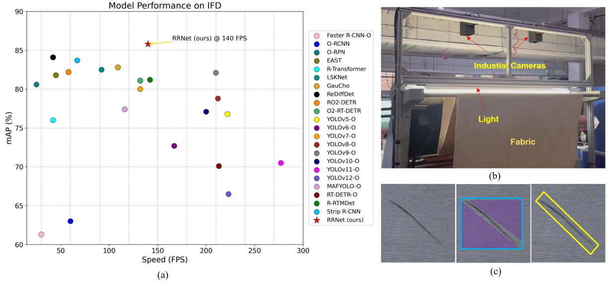
Fig. 1. Accuracy–throughput comparison, online inspection scenario, and annotation comparison for IFD detection. (a) Accuracy–throughput comparison on the IFD dataset, where RRNet achieves the best accuracy–efficiency tradeoff among the compared methods. (b) Line-scan inspection system for online fabric defect detection. (c) Comparison between horizontal and rotated bounding-box annotations. Horizontal boxes contain substantial redundant background for elongated and tilted defects, whereas rotated boxes provide tighter geometric localization.
