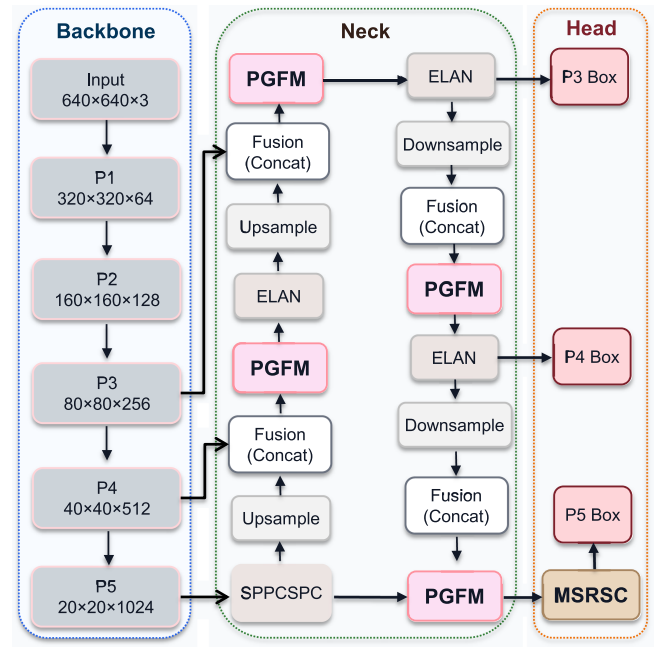
Fig. 2. Overall architecture of RRNet. PGFM preserves defect-consistent spatial evidence through postfusion recalibration at selected neck nodes, while MSRSC strengthens the P5 branch with structure–direction coupling for rotated defect prediction.
