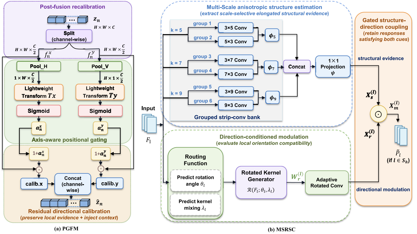
Fig. 3. Architectures of PGFM and MSRSC. (a) PGFM recalibrates postfusion features to preserve defect-consistent spatial evidence after cross-scale aggregation. (b) MSRSC separates anisotropic structure estimation from direction-conditioned modulation and couples them through multiplicative gating for structure–direction consistent rotated prediction.
