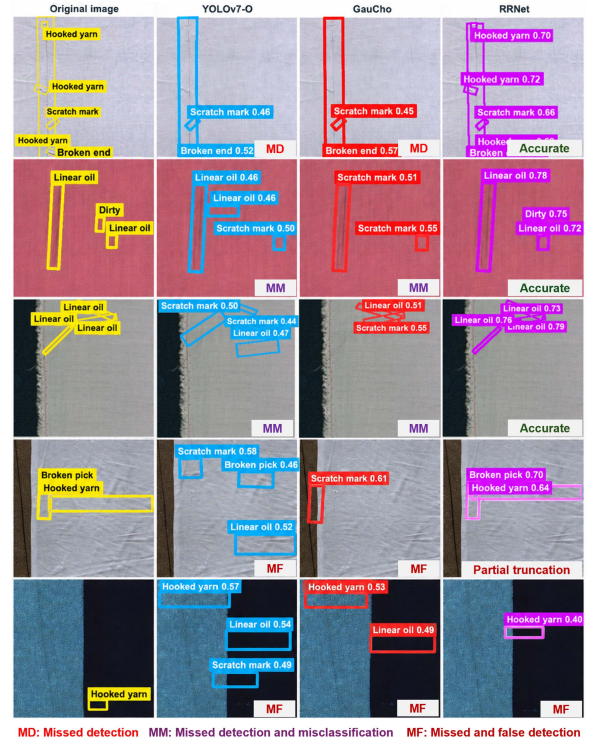
Fig. 4. Qualitative detection comparisons on the IFD dataset under different scenarios. Rows 1–3 show multifect and cluttered-background scenarios, while Rows 4 and 5 show representative failure cases. Compared with the YOLOv7-O baseline and GauCho, RRNet reduces missed detections and category confusion and achieves more complete rotated localization, although small and low-contrast defects remain challenging.
